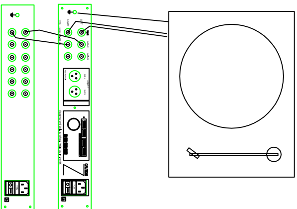
Fig 2. Basic Audio Connection —Ground connection
